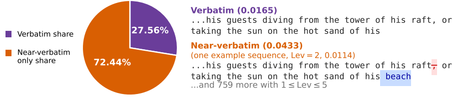
Figure 6: Verbatim share. For LLAMA 2 7B and one sequence from The Great Gatsby , we show the verbatim share (Equation 7): 27.56% of the total near-verbatim mass \hat{p}_{z,5}^{\text{Lev}} \approx 0.06 .
