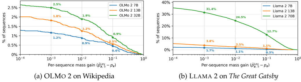
Figure 5: CCDF of per-sequence near-verbatim mass gain. For Lev \varepsilon = 5 mass minus verbatim mass ( \hat{p}_{z,5}^{\text{Lev}} - p_z ), a point (x, y) means y\% of sequences have extraction-mass gain \geq x .
