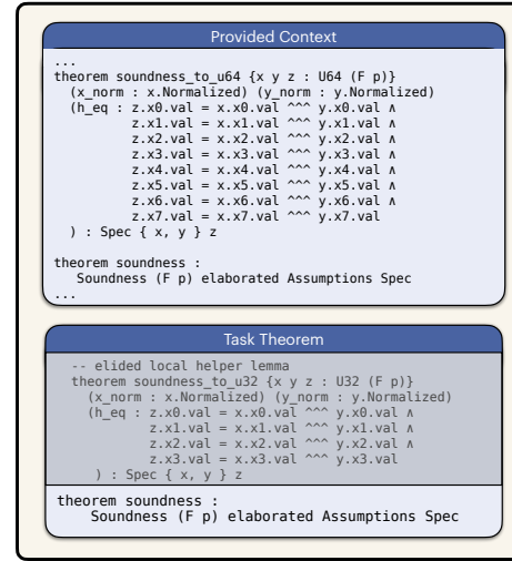
Figure 5: Full-repository context exposes the analogous soundness_to_u64 proof as a pattern for the target soundness_to_u32; curated context omits it.
