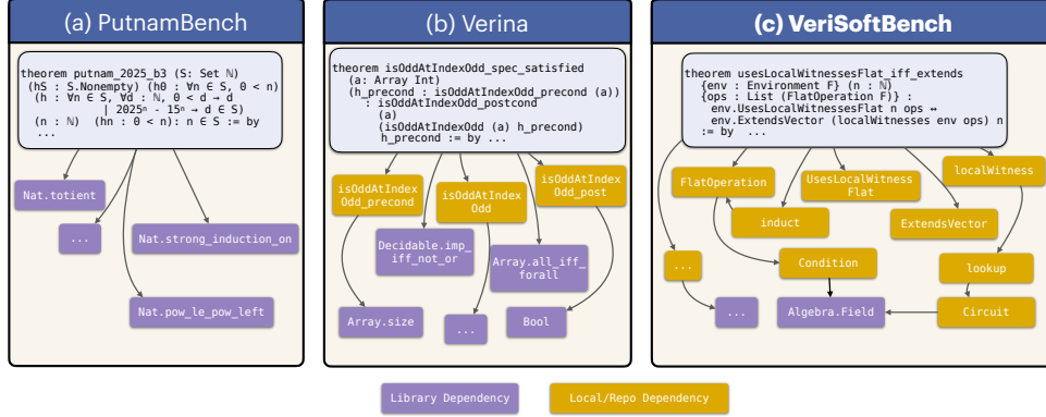
Figure 1: Contextual dependencies comparison between (a) mathematical benchmark proofs, (b) lightweight verification tasks, and (c) repository-scale verification. PutnamBench proofs rely almost entirely on library (Mathlib) dependencies (purple). Verina introduces a small number of project-specific definitions (yellow) but remains largely library-driven. In contrast, proofs from a real-world ZK circuit DSL repository (Verified-zkEVM, 2025) depend heavily on interconnected local abstractions, forming a dense repository-level dependency graph. Purple denotes library dependencies; yellow denotes local/repository dependencies.
