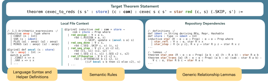
Figure 3: An example VeriSoftBench task. The target cexec_to_reds relates two project-defined execution relations. The left (local-file) panel supplies the language syntax and semantic rules in scope at the theorem; the right (repository) panel supplies cross-file base types and relational lemmas. Matching colors trace each project-specific symbol in the target to the declaration that gives it meaning, illustrating why the proof cannot be treated as an isolated theorem statement.
