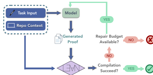
Figure 4: Evaluation pipeline.
