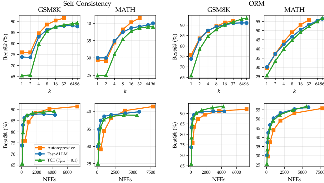
Figure 11: Test-time scaling for LLaDA-8B-Instruct in terms of Best@ k (top) and Best@NFE (bottom) when using either self-consistency or an ORM for final answer selection. TCT performs worse compared to AR at higher NFEs when using self-consistency; however, when using an ORM, TCT improves the Pareto frontier compared to autoregressive rollouts.
