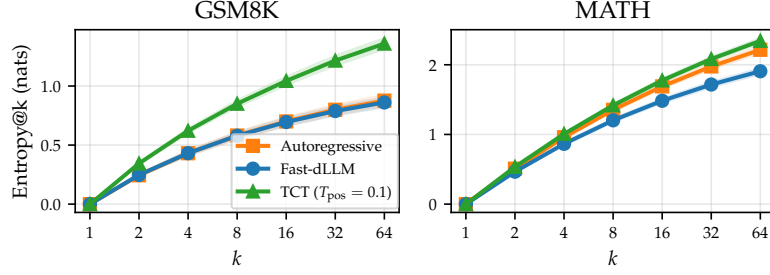
Figure 12: Mean empirical entropy of the per-question answer distributions (see Figure 13) as a function of the group size k . TCT consistently yields higher-entropy answer distributions than autoregressive and confidence thresholding, particularly on GSM8K.
