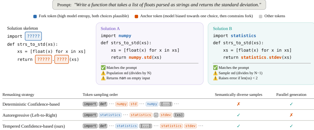
Figure 1: An example illustrating our model of entropy degradation. The fork token (Definition 1) has high marginal uncertainty under the dLLM, indicating that both the numpy and statistics solutions are plausible. However, the dLLM is simultaneously overly confident in its prediction at the anchor tokens in the function body, biasing low-confidence remasking towards one solution as it reveals those tokens first. Tempered remasking allows the fork to still be revealed first, increasing semantic diversity without sacrificing parallelism. Note that while both paths lead to generations that match the prompt (✓), they have subtly different semantics (⚠); sampling both is important to achieve good coverage.
