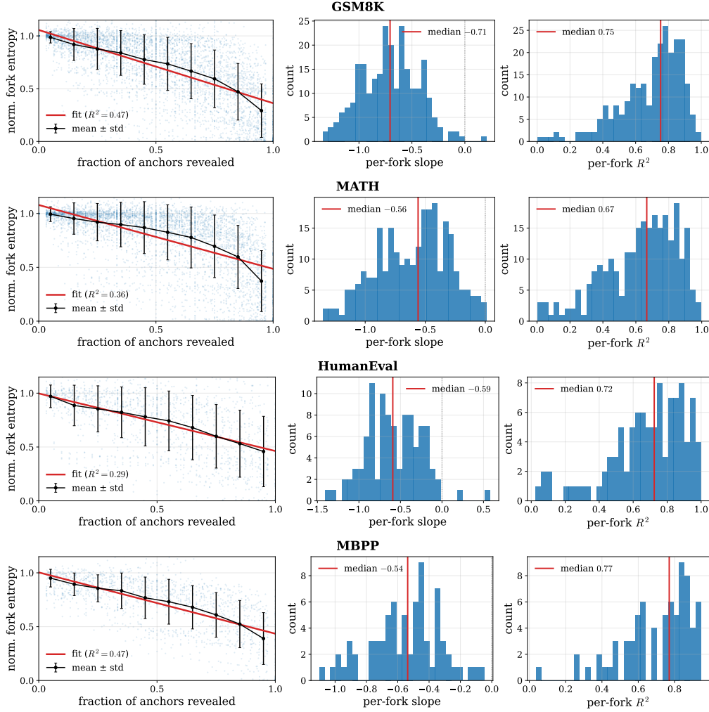
Figure 6: Empirical validation of Assumption 1. Left : Entropy degradation at potential fork tokens as a function of how many potential anchors have been revealed, aggregated over all forks and samples. Middle : Slopes of per-fork linear fits. Right : R^2 correlation between each fork’s entropy degradation and a linear fit on that fork’s data. In all cases, we see that forks tend to decrease in entropy as their anchors are revealed. While different forks vary in how much their entropies change (causing large error bars and lower R^2 on the left), most exhibit an internally nearly-linear relationship (the median per-fork R^2 being \sim 0.7 across datasets in the rightmost plot), and almost all decrease in entropy (middle).
