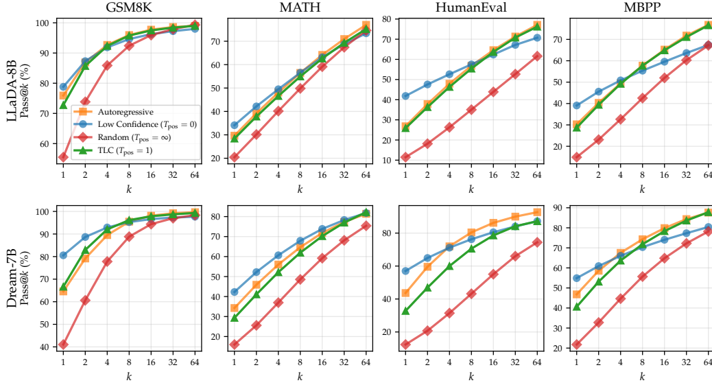
Figure 2: Pass@ k for TLC ( T_{\text{pos}} = 1 ) on LLaDA-8B-Instruct and Dream-7B-Instruct across four benchmarks. TLC closely tracks the AR baseline, recovering almost all of the diversity lost by low-confidence remasking.
