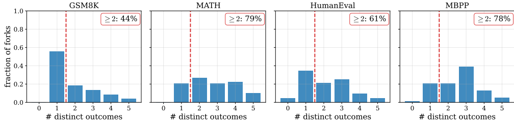
Figure 7: Number of semantically distinct and well-formed outcomes when setting a fork position from Figure 6 to each of its top 5 most likely values. Overall, a majority of the fork positions produce \geq 2 valid and semantically distinct outcomes, indicating that they play an important role in determining the semantics of the outcome (rather than just syntax).
