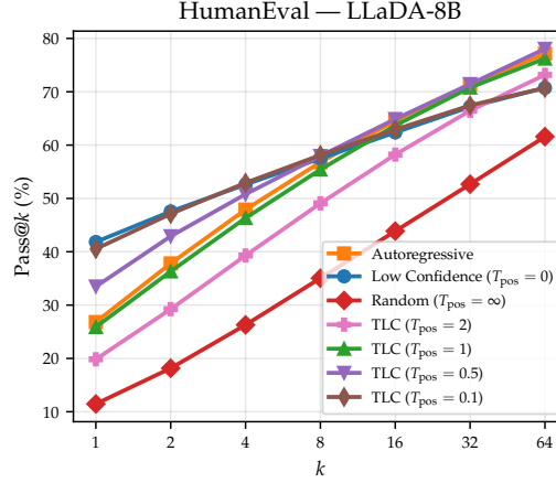
Figure 8: TLC T_{\text{pos}} ablation on HumanEval with LLaDA-8B-Instruct at T_{\text{token}} = 0.8 . Too little tempering ( T_{\text{pos}} = 0.1 ) remains close to low-confidence remasking, while too much ( T_{\text{pos}} = 2 ) approaches random remasking and degrades quality. Intermediate values ( T_{\text{pos}} \in \{0.5, 1\} ) strike the best balance, matching or exceeding the autoregressive baseline at high k .
