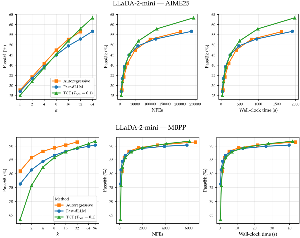
Figure 15: Pass@ k and pass@NFE for TCT on LLaDA-2-mini (Bie et al., 2025). In addition to pass@ k (Left) and pass@NFE (Middle), we here additionally report pass@wall-clock-time (Right) to show that our proposed TCT has a negligible overhead in terms of latency compared to Fast-dLLM.
