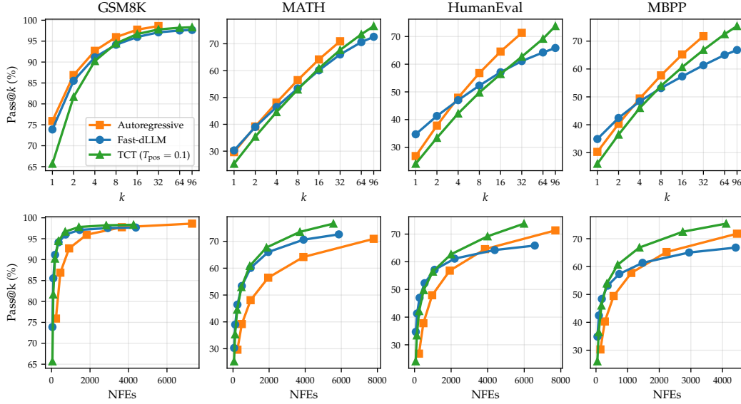
Figure 3: Pass@ k (top) and pass@NFE (bottom) for TCT on LLaDA-8B-Instruct. Both rows plot the same data; only the metric changes (pass@ k vs pass@NFE). TCT slightly underperforms AR in pass@ k , but substantially outperforms it when the cost of each sample is taken into account. TCT also outperforms deterministic confidence-thresholding (Fast-dLLM; Wu et al. 2026a) thanks to its additional source of randomness via T_{\text{pos}} .
