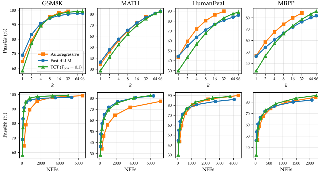
Figure 10: Pass@ k (top) and pass@NFE (bottom) for TCT on Dream-7B-Instruct. Note that both rows plot the same data, we just vary the x-axis measure ( k vs NFEs). While TCT slightly underperforms AR in pass@ k , it outperforms AR when the cost of each rollout is taken into account.
