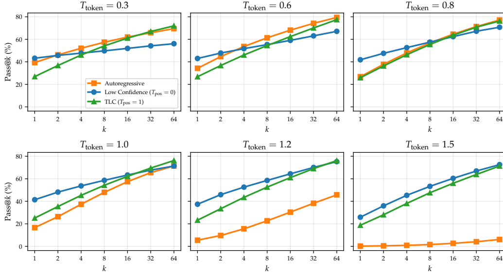
Figure 9: Varying T_{\text{token}} for LLaDA-8B-Instruct on HumanEval. Autoregressive generation favors low temperatures, obtaining its best pass@64 at T_{\text{token}} = 0.6 . Meanwhile, low-confidence remasking scales very poorly at low token temperatures due to its greedy position selection. TLC consistently shows strong scaling and most robustness to the exact choice of T_{\text{token}} , matching or exceeding the best of autoregressive and low-confidence remasking in pass@64 at all temperatures. Moreover, it exhibits stronger scaling compared to low-confidence across all considered T_{\text{token}} , suggesting it achieves diversity through an alternative mechanism.
