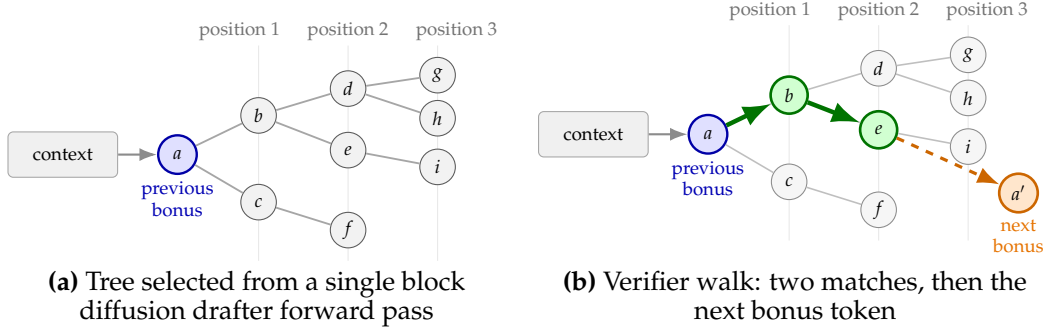
Figure 2: Illustration of one DDTree decoding round. The bonus token a from the previous round is carried into the current round and serves as the tree root. One block diffusion drafter pass produces per-position marginals for the next three draft positions, from which DDTree selects a draft tree. During verification, the target model follows its own decoding rule, and the walk continues whenever the selected token appears as a child in the tree. In this example, two speculative nodes are matched (green), the matched path is added to the output, and the first unmatched target token a' becomes the bonus token for the next round.
